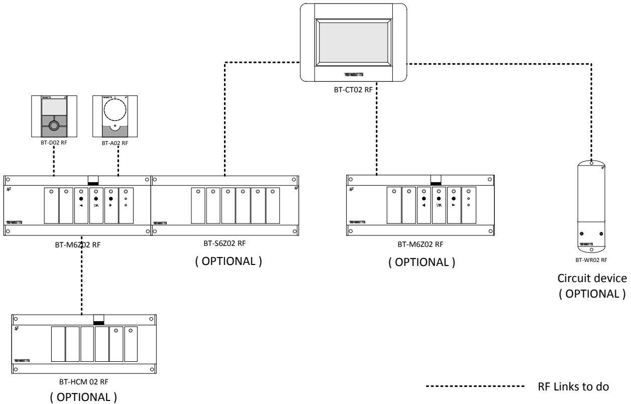
Exemple of an “Centralized Installation”
